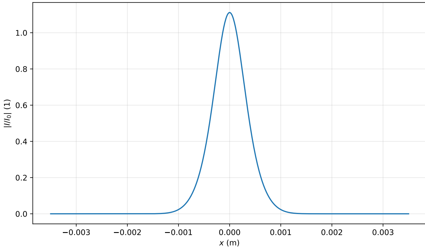
Intensity profile I(x, y = 0, z = 0.796m)/I_0 , P_{in}=0.6P_{cr} , artificial time
